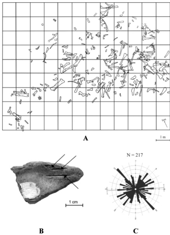
Fig. 6 A: map of the Blagoveschensk bonebed made during 2005 field campaign. B: dentary fragment displaying sub-parallel grooves, interpreted as predator or scavenger tooth marks. C: mirror rose diagrams with 5° petals for bones recovered at Blagoveschensk in 2005
