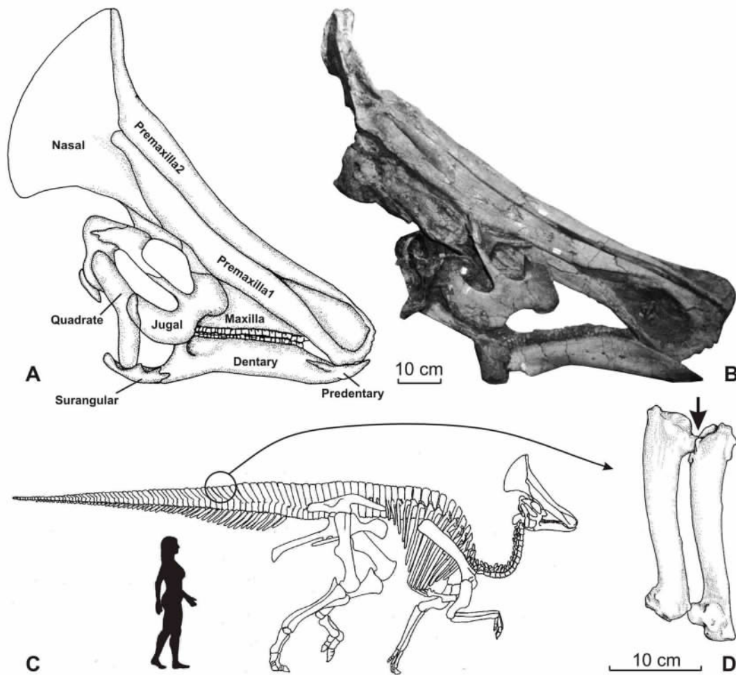
A: reconstruction of the skull in right lateral view ( only bones that have been discovered are labelled) . B: main part of the skull of the holotype AEHM 2/845 in right lateral view ( some deformation results from lateral compression of the skull) ; the largest part of the nasals , the maxillae , the surangulars , the left dentary and the predentary were found disconnected from this piece and are therefore not represented in this photograph. C: full skeletal reconstruction based on holotype AEHM 2/845. D: detail of the neural spines of the proximal caudal vertebrae , displaying the additional articulation.
