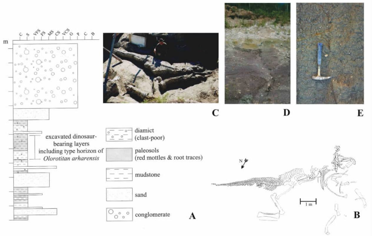
Fig. 9 A: lithostratigraphy of Exposure 18 at Kundur ( Russia ) on the opposite side of the road of the main dinosaur site. B: sketch of the Olorotitan skeleton excavated during summer of 2000 and 2001. C: picture of part of the Olorotitan skeleton excavated during summer of 2000. D: dystric argillisol at the top of the Udurchukan Formation ( depth of the soil profile = 2m ) . E: detail of dinosaur bearing clast-poor diamictite
