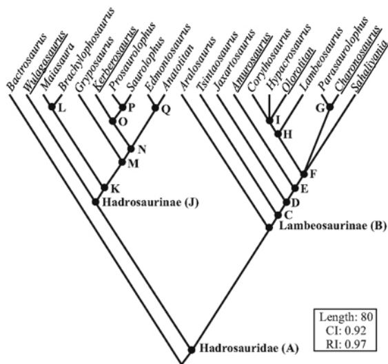
Fig. 13 Phylogenetic relationships of Hadrosauridae (Taxa found in the Amur/Heilongjiang region are underlined. Letters correspond to nodes defined in Appendix 3)
