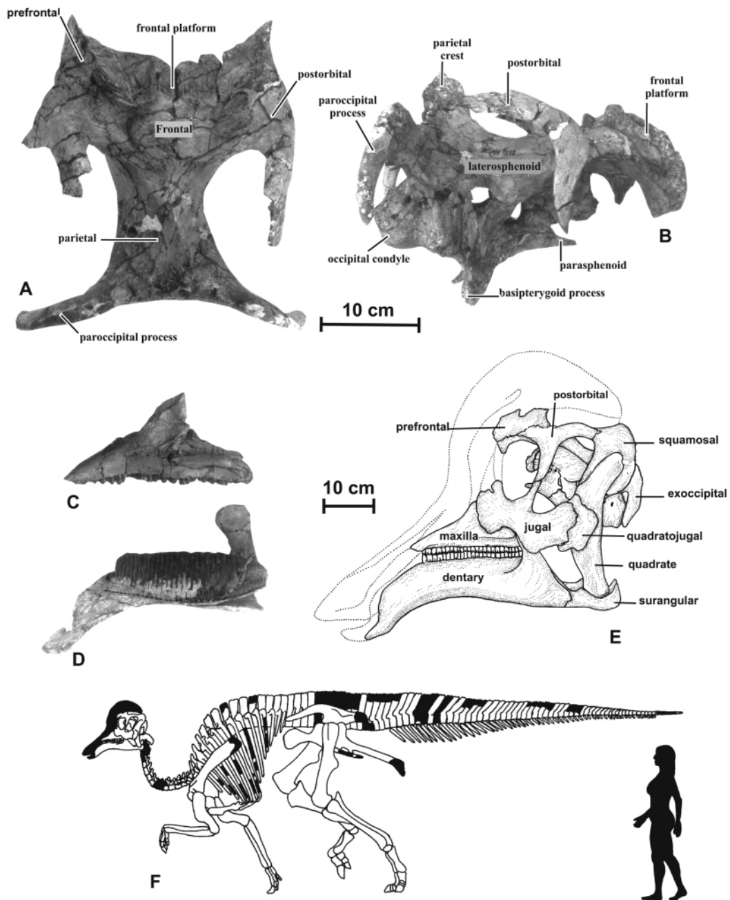
A-B: braincase ( AEHM 1/232 ) in dorsal ( A ) and right lateral ( B ) views. C: left maxilla ( AEHM 1/12 ) in lateral view. D: left dentary ( AEHM 1/12 ) in medial view. E: reconstruction of the skull in left lateral view. F: reconstruction of the whole skeleton.
