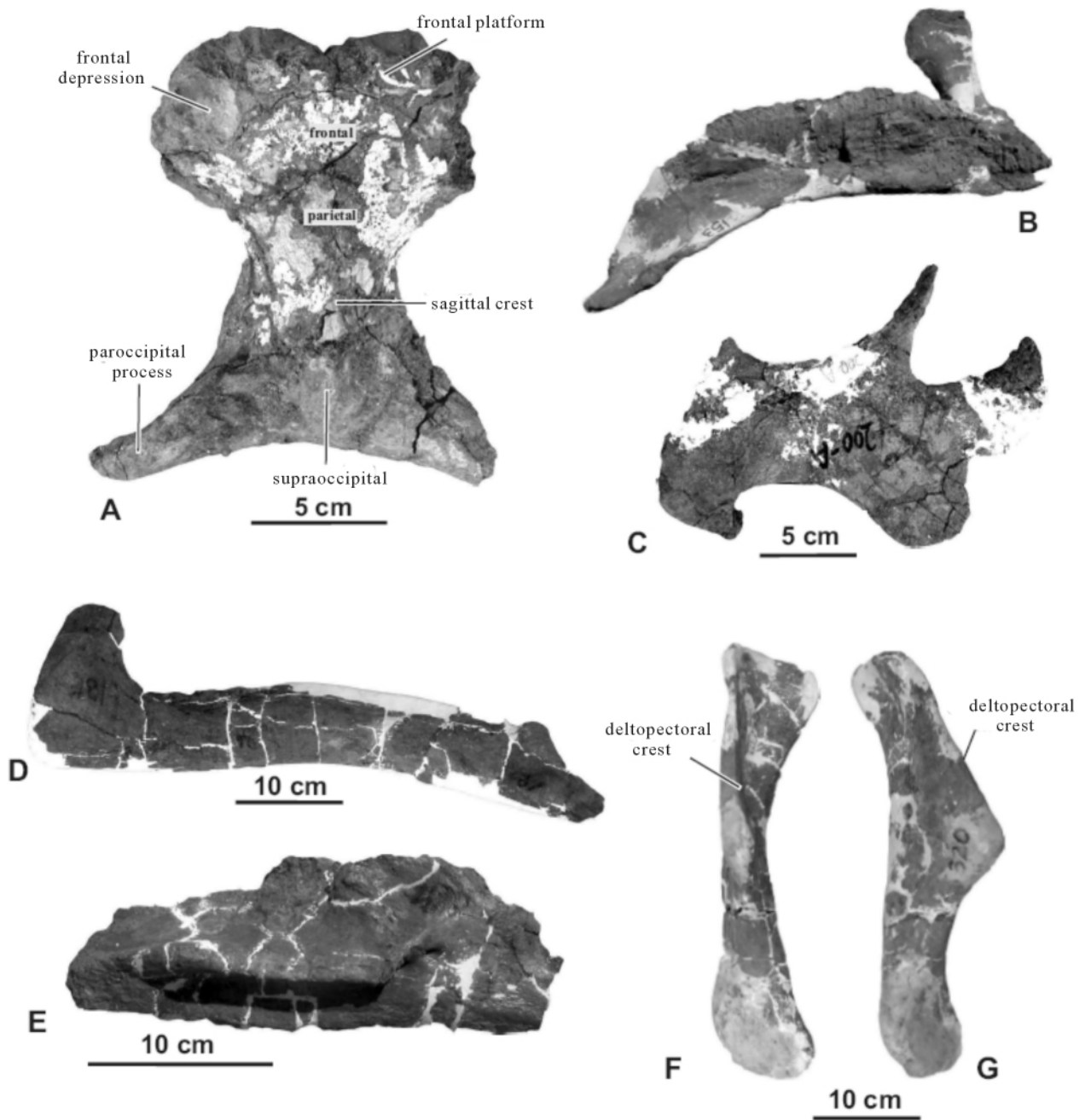
A: Braincase of Sahaliyania elunchunorum (GMH W453) in dorsal view. B: right dentary of Sahaliyania elunchunorum (GMH W153) in medial view. C: left jugal of Sahaliyania elunchunorum (GMH W200-A) in lateral view. D: right dentary of Wulagasaurus dongi (GMH W184) in lateral view. E: right maxilla of Wulagasaurus dongi (GMH W400-10) in lateral view. F-G: right humerus of Wulagasaurus dongi (GMH W320) in cranial (F) and medial (G) views
