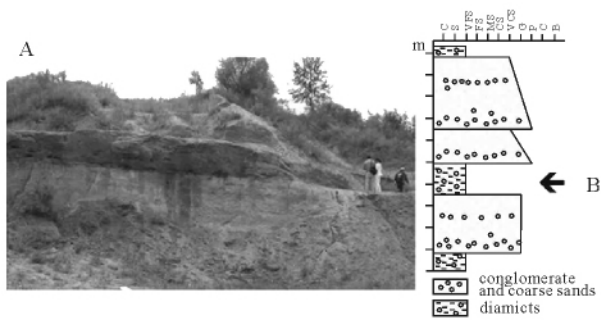
Fig. 11 A: Wulaga dinosaur site ( China ) , peoples on the right hand side of the picture are standing on the excavated surface. B: Lithostratigraphic column of the Wulaga dinosaur site , black arrow indicates dinosaur-bearing horizon
