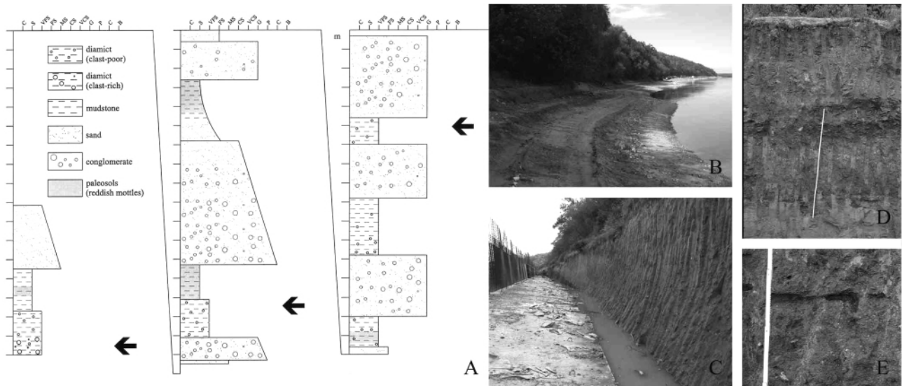
Fig. 3 A: lithostratigraphy of the Longgushan section ( Jiayin , China ) , black arrows indicate the excavated dinosaur-bearing layers. B: view on the Longgushan section along the right side of the Amur River. C: view on temporary outcrop behind concrete cliff protection. D: sediments of the Yuliangze Formation with reddish-purple palaeosol horizons. E: diamictite layer with black dinosaur bones
