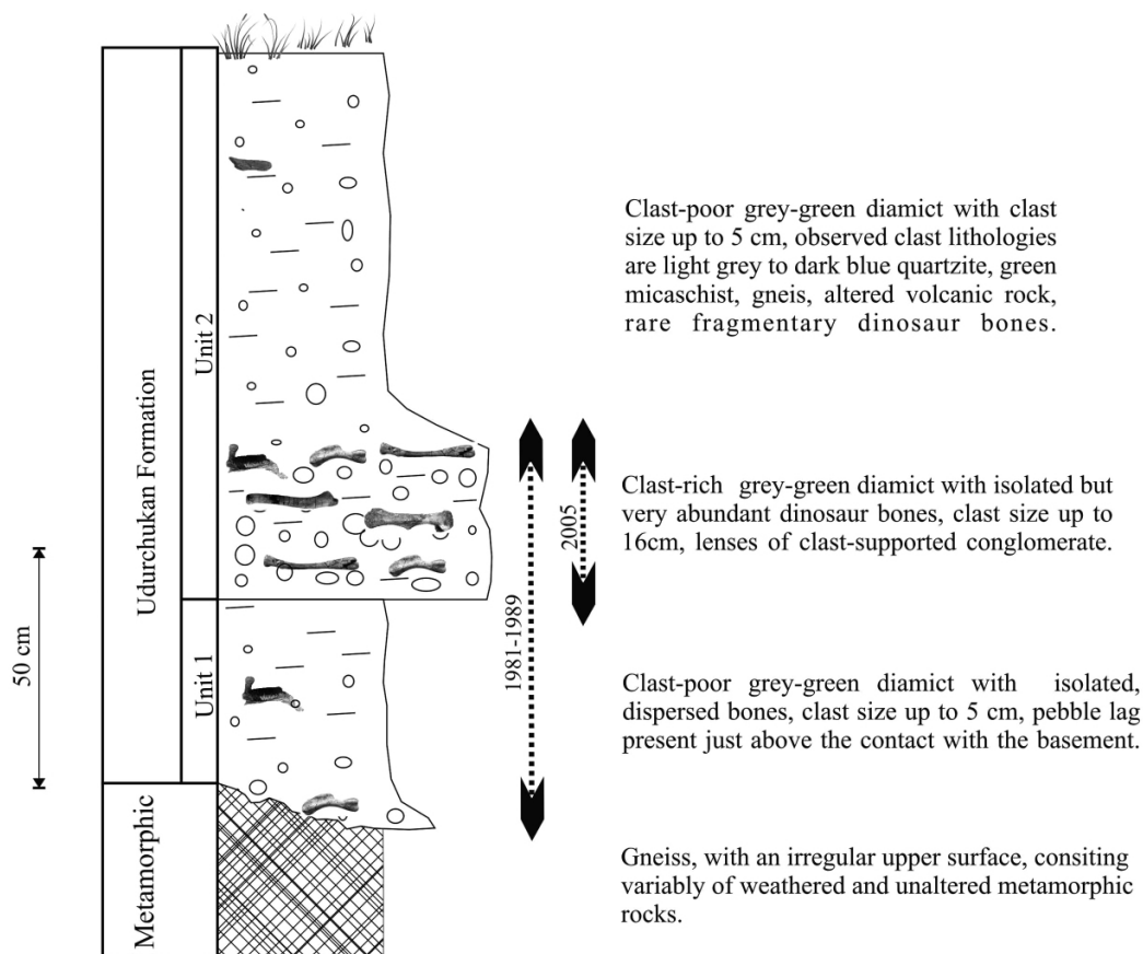
Fig. 5 Stratigraphic section of the dinosaur locality at Blagoveschensk ( Russia) . Black arrows indicate the excavated layers
